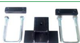
Holder for front loosener share, without spring-loaded front loosener share, for Fendt GT 231
