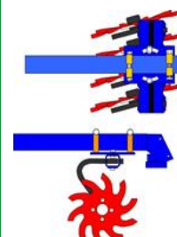
Star cultivator tool kit maize, half 4 stars (red OR black) incl. tube and brackets
